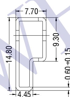
4 Pin SIP Tube
