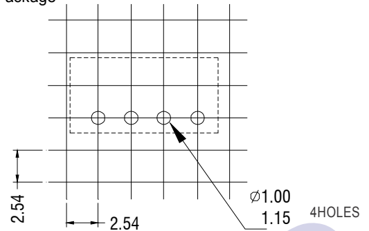
4 Pin SIP Package
