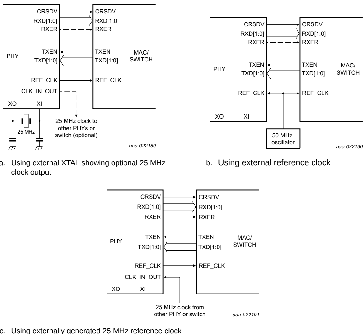
Fig 5. RMII signaling
