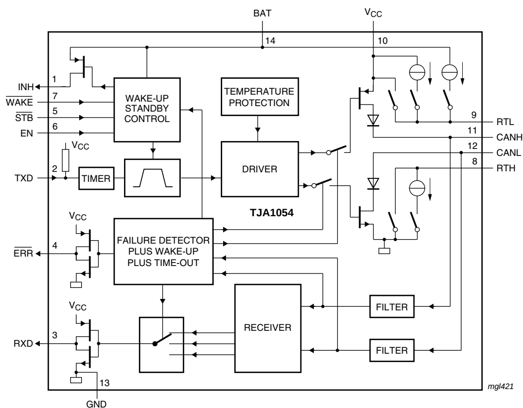
Fig 1. Block diagram
