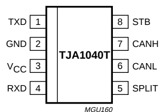
Fig.2 Pin configuration.
