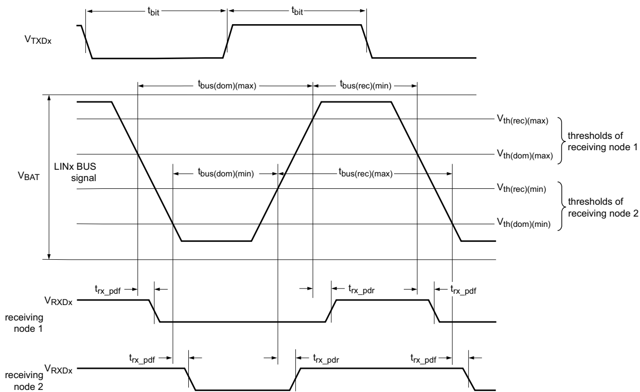
Fig 6. Timing diagram of LIN transceiver duty cycle
