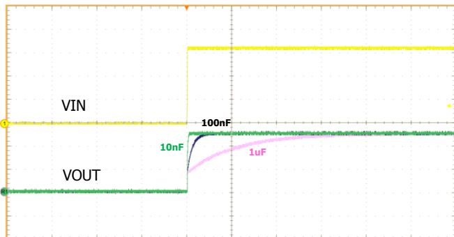
Start Up @ Iout=1A (Cff is varied, R2=51KΩ, R1=24KΩ)
