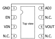
DFN2X3-8L
