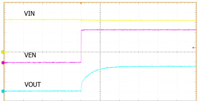
Start Up by external VEN @ Iout=1A (Cff=10nF, R2=51KΩ, R1=24KΩ)
