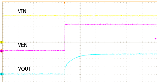
Start Up by external VEN @ Iout=0A (Cff=10nF, R2=51KΩ, R1=24KΩ)
