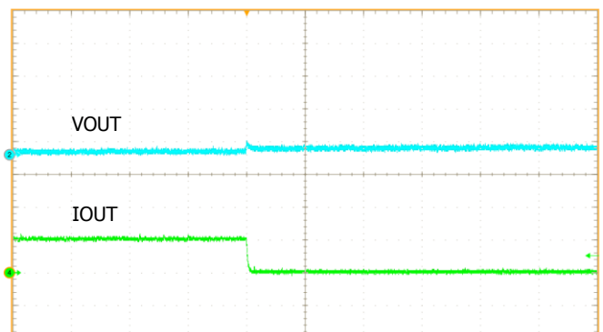
Load Transient Response (Cff=10nF, R2=51KΩ, R1=24KΩ)
