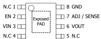
SOP8/SOP8-PP
