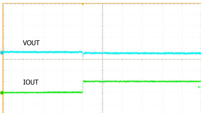
Load Transient Response (Cff=10nF, R2=51KΩ, R1=24KΩ)
