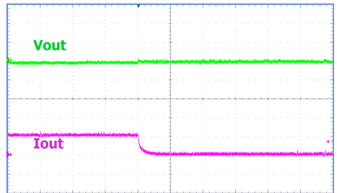
Load Transient Response (Cff =10nF, R2=51K \Omega , R1=24K \Omega )
