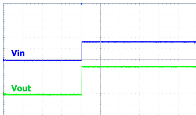
Start Up @ Iout=300mA (Cff=10nF, R2=51KΩ, R1=24KΩ)
