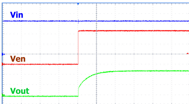
Start Up @ Iout=0A (Cff=10nF, R2=51K \Omega , R1=24K \Omega )
