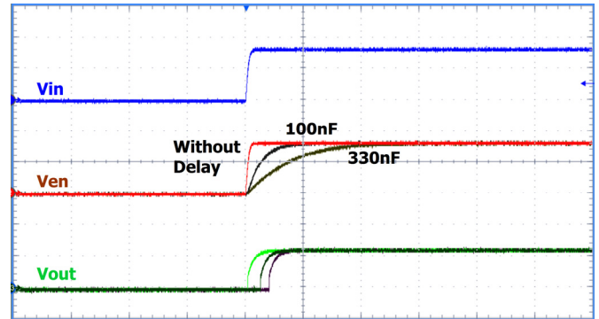
Start Up @ Iout=10mA (Cff is varied, R2=51K \Omega , R1=24K \Omega )
