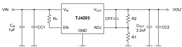
Fig. 2. Application with Feed-Forward Capacitor, CFF
