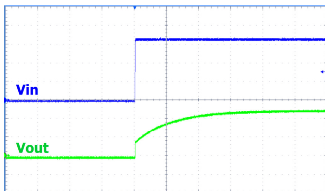
Start Up @ Iout=300mA (Cff=1uF, R2=51KΩ, R1=24KΩ)
