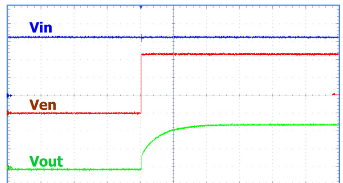
Start Up @ Iout=300mA (Cff=10nF, R2=51K \Omega , R1=24K \Omega )
