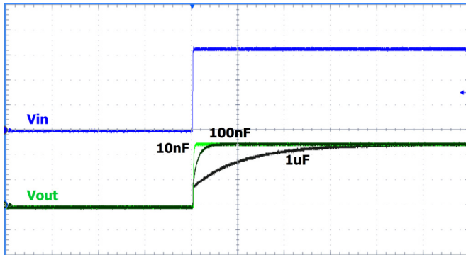
Start Up @ Iout=300mA (Cff is varied, R2=51K \Omega , R1=24K \Omega )
