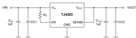
Fig. 1. Application with Decoupling Capacitor, CC1 & CC2
