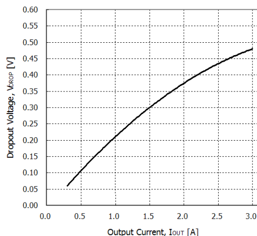
Output Current vs. Dropout Voltage
