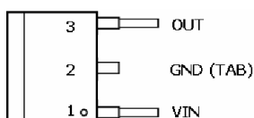
TO252-3L
