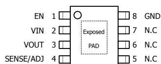
SOP8-PP (Exposed PAD)
