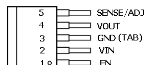
TO252-5L
