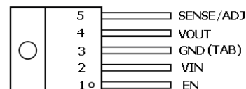
TO220-5L
