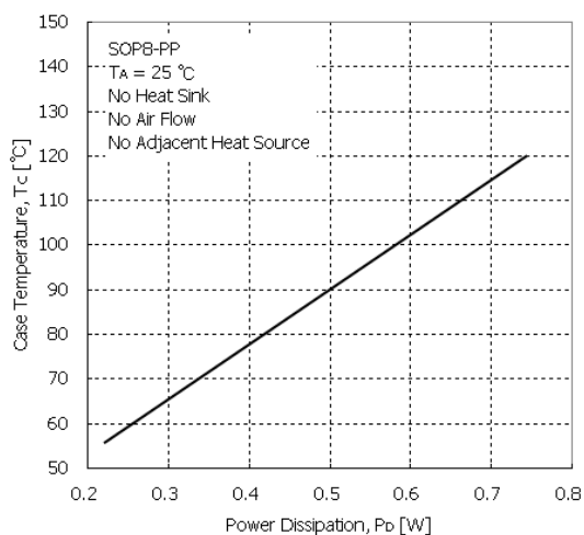
Power Dissipation vs. Case Temperature, SOP8-PP
