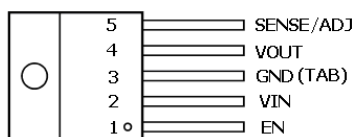
TO220-5L
