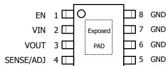
SOP8-PP(Exposed PAD)
