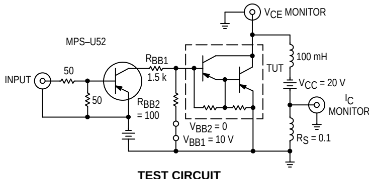
TEST CIRCUIT
