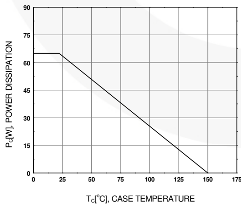
Figure 5. Power Derating
