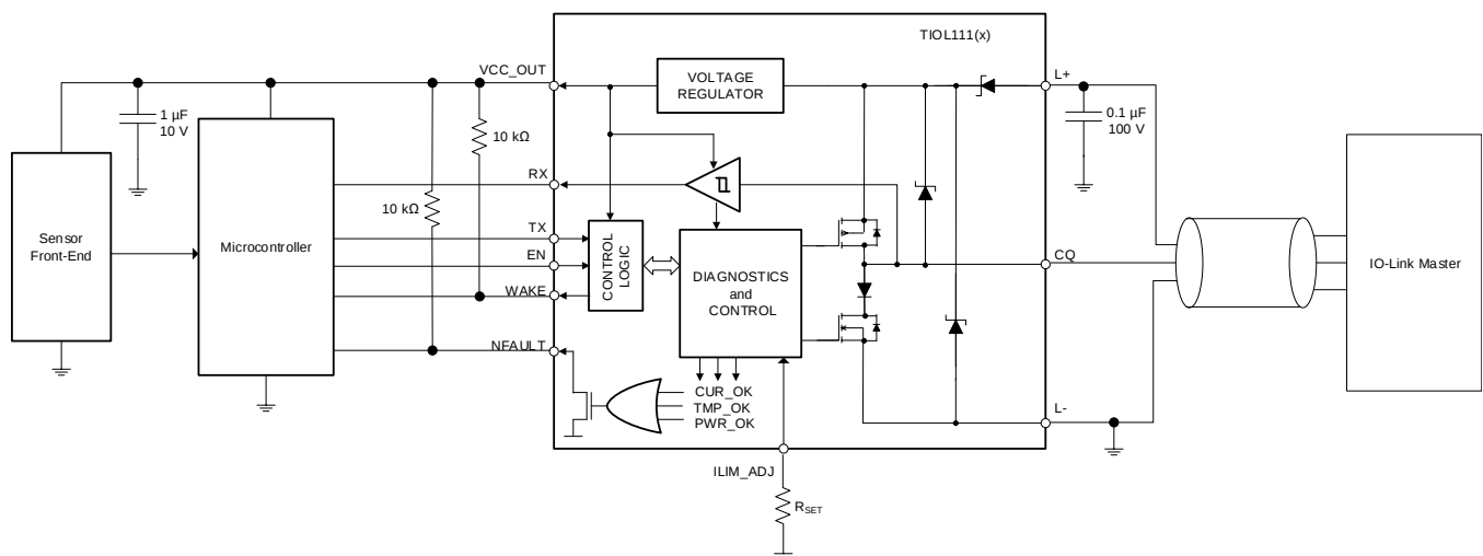
Figure 17. Typical Application Schematic
