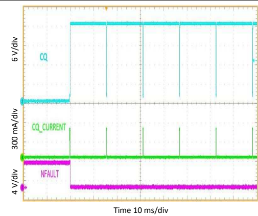
Figure 25. CQ in Current Fault Auto Recovery, Low Side Mode
