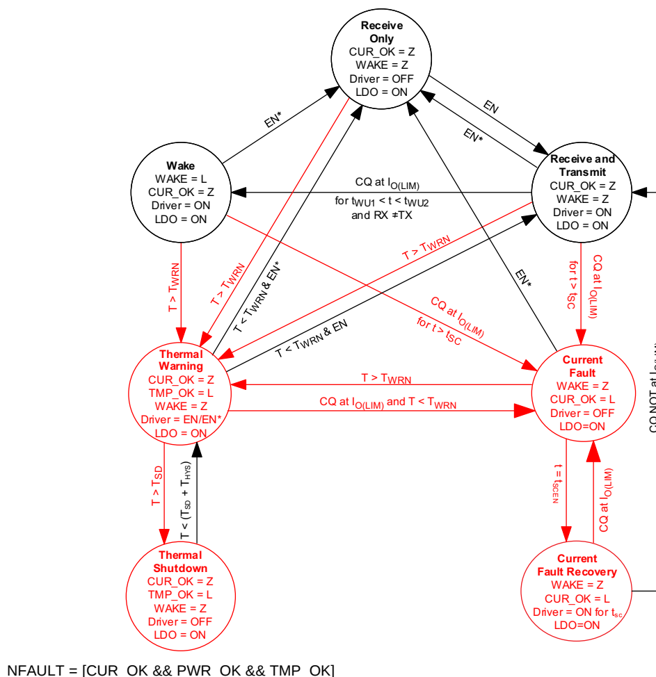
Figure 13. Device State Diagram
