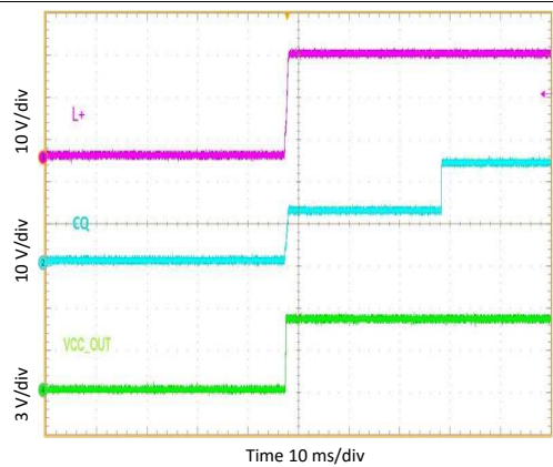
Figure 20. CQ in Communication Mode
