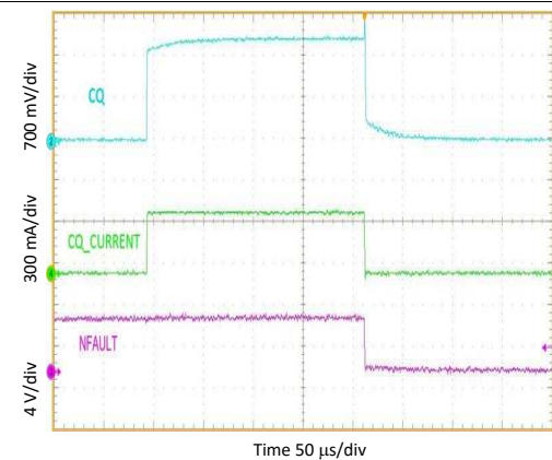
Figure 21. CQ Power Up Delay, Low Side Mode
