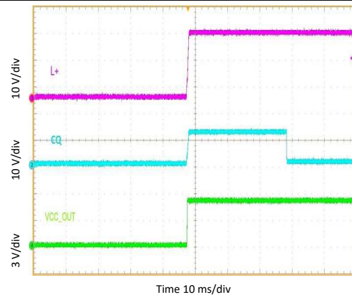
Figure 21. CQ Power Up Delay, Low Side Mode
