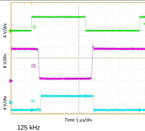
Figure 20. CQ in Communication Mode
