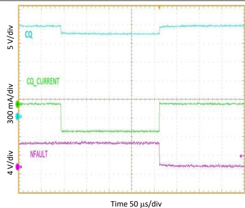
Figure 22. CQ Power Up Delay, High Side Mode
