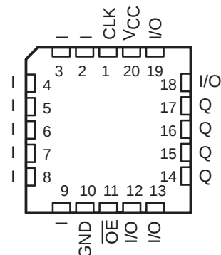
TIBPAL16R4' C SUFFIX ... FN PACKAGE M SUFFIX ... FK PACKAGE
