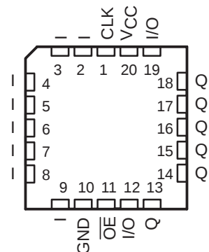
TIBPAL16R6' C SUFFIX ... FN PACKAGE M SUFFIX ... FK PACKAGE
