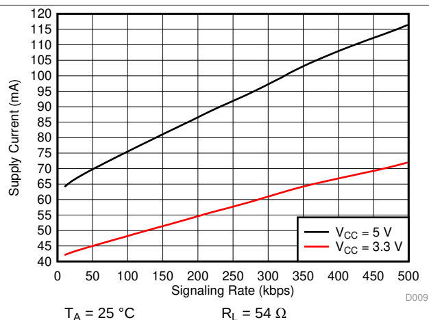
Figure 6. THVD2410 Supply Current vs Signal Rate
