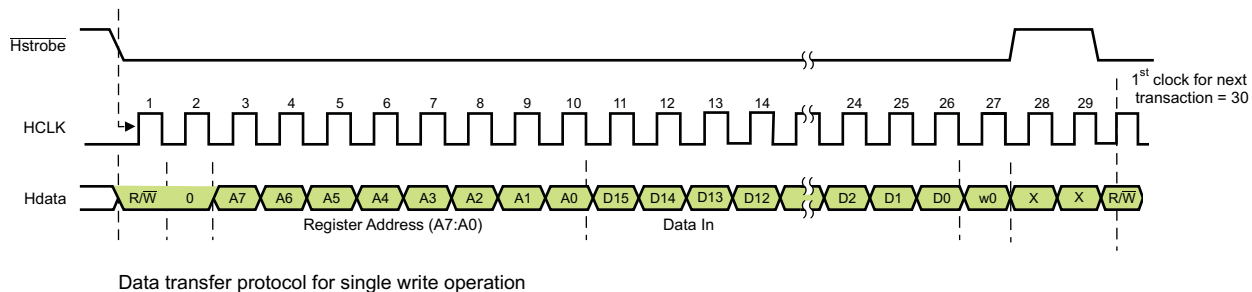
Figure 4. Write Operation
