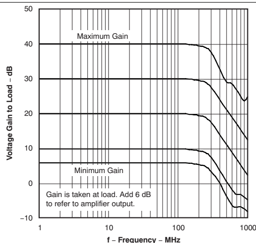
Figure 1. Voltage Gain to Load vs Frequency ( P_{IN} = -45 dBm)
