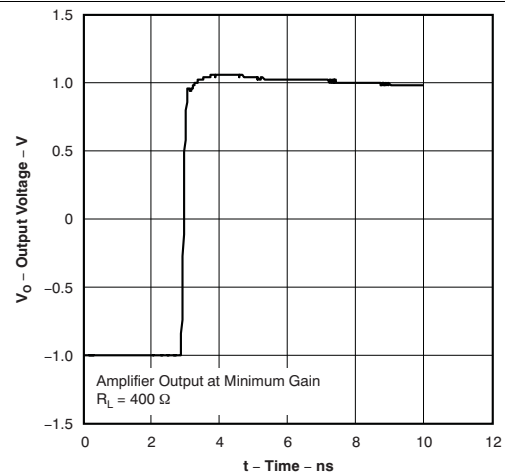
Figure 14. Step Response: Rising Edge
