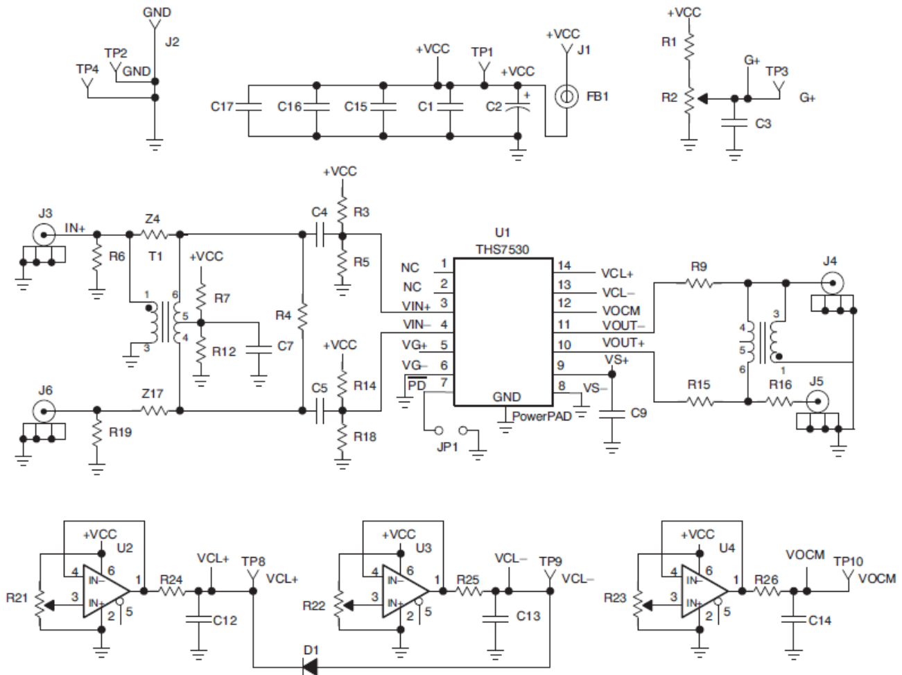
Figure 27. EVM Schematic
