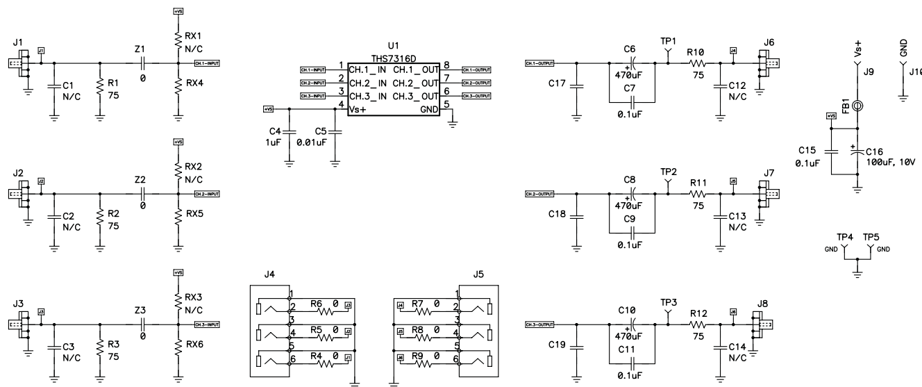
Figure 33. THS7316D EVM
