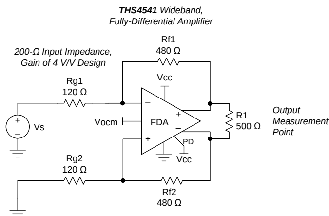
Figure 72. 200- \Omega Input Impedance, Single-Ended to Differential DC-Coupled Design with Gain of 4 V/V
