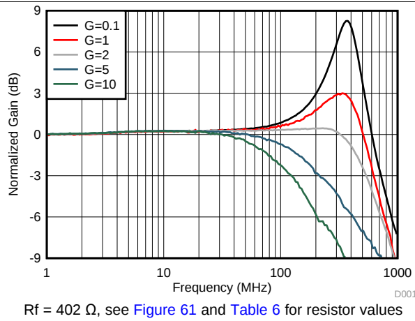
Figure 1. Small-Signal Frequency Response vs Gain
