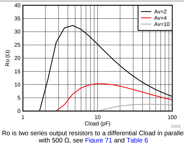
Figure 6. Recommended R_o vs Load
