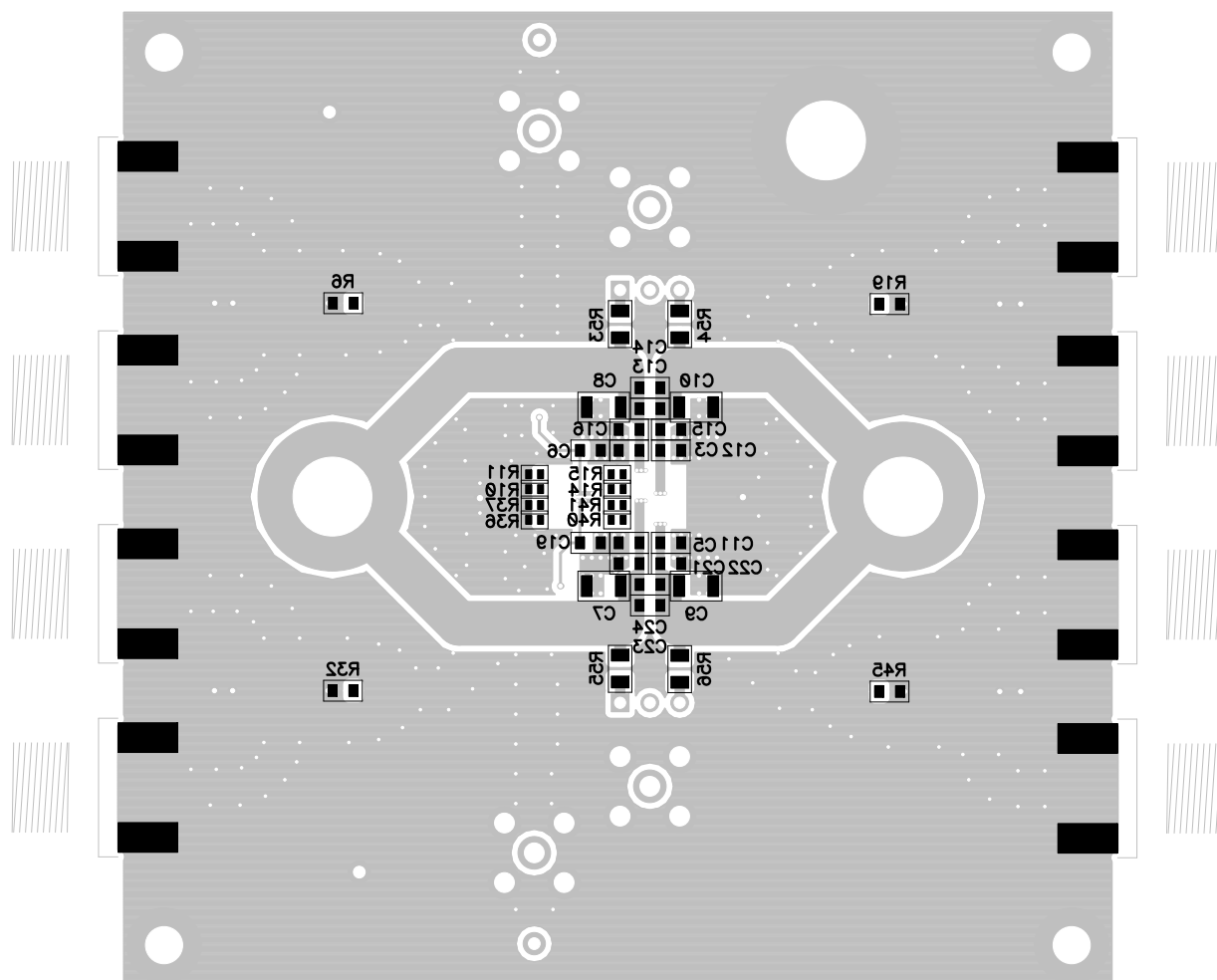
Figure 6. THS4532 EVM Bottom Layer 4
