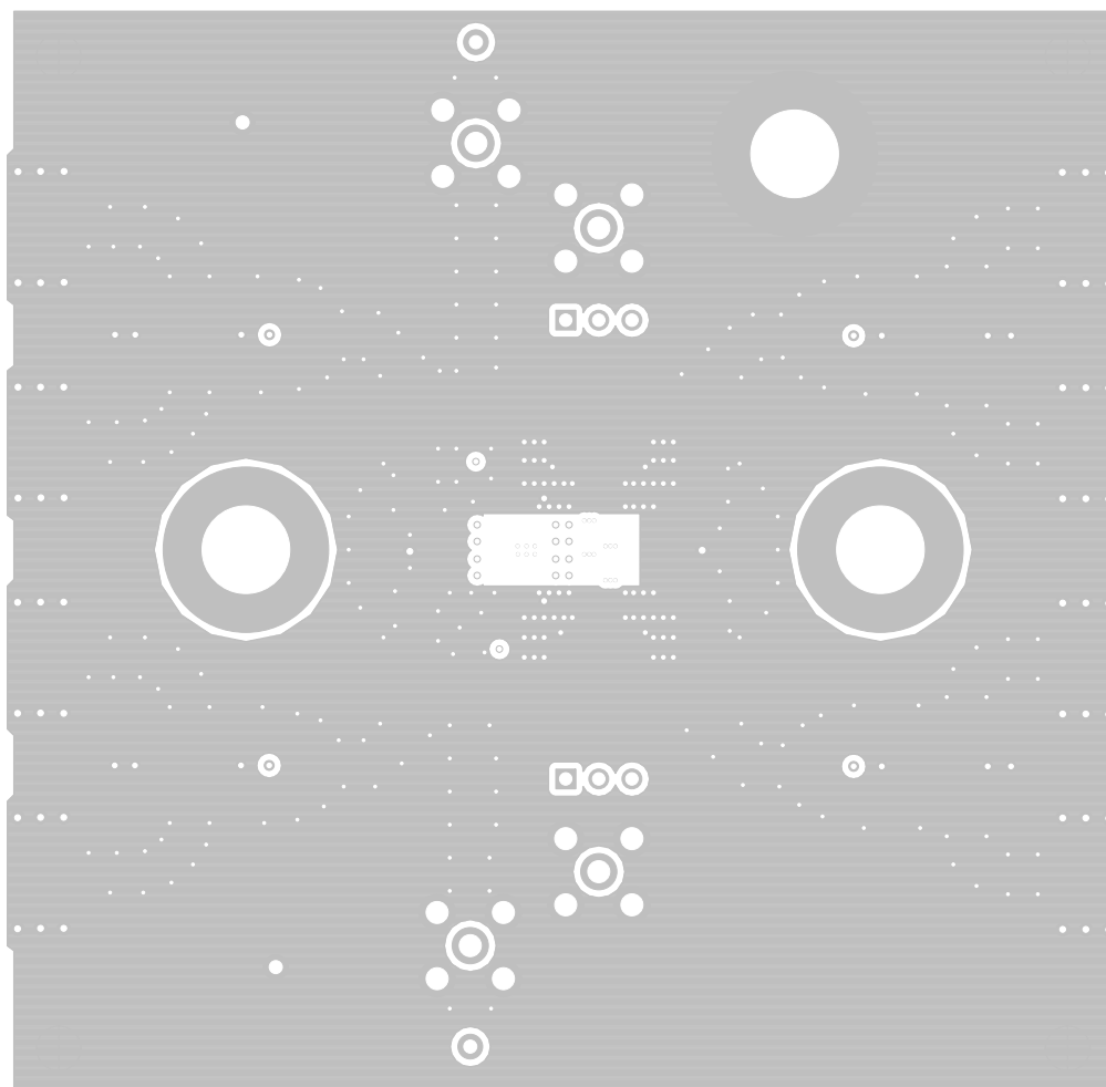
Figure 5. THS4532 EVM Ground Layer 3
