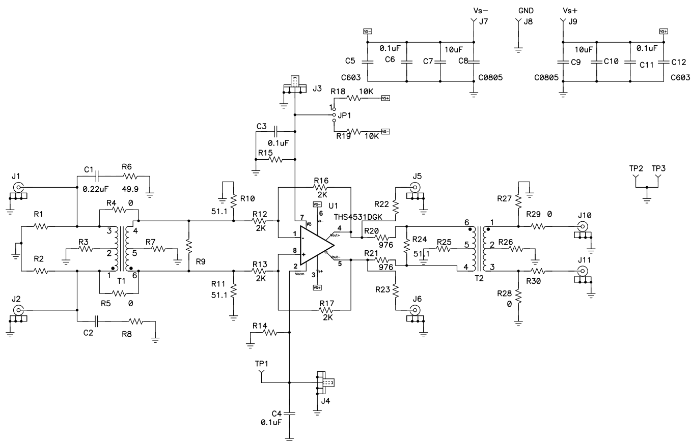
Figure 1. THS4531ADGKEVM Schematic
