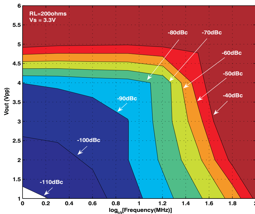
Figure 70. Constant HD2 Contours vs Output Swing and \log_{10} (Frequency - MHz) V_s = 1.65 V , Gain = 1, R_L = 200 \Omega
