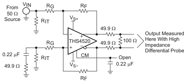
Figure 56. Frequency Response Test Circuit
