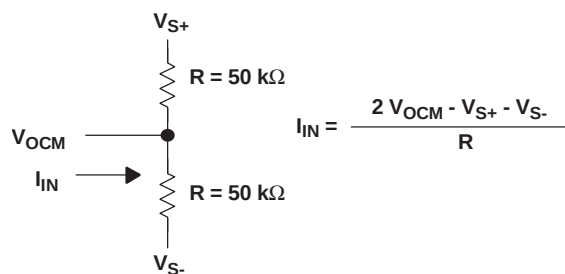
Equivalent Input Circuit for V_{OCM}
