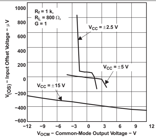
Figure 26. Input Offset Voltage vs Common-Mode Output Voltage
