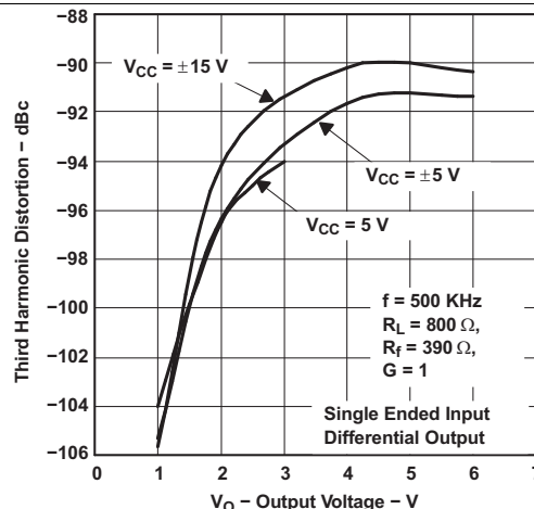
Figure 22. Third-Harmonic Distortion vs Output Voltage
