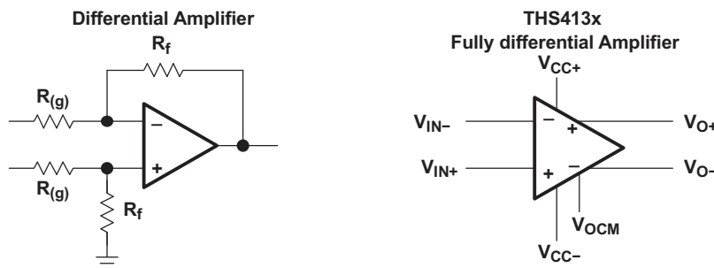
Figure 29. Differential Amplifier Versus a Fully-Differential Amplifier
