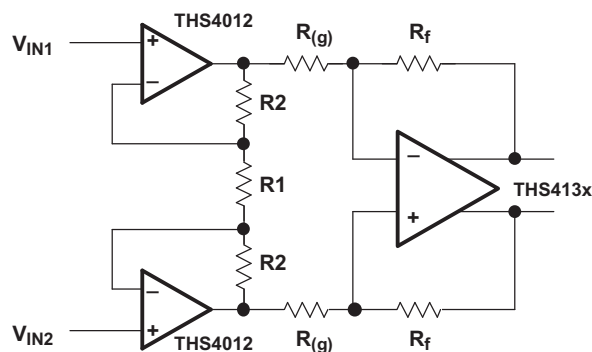
Figure 32. Instrumentation Amplifier
