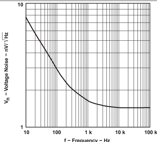
Figure 24. Voltage Noise vs Frequency
