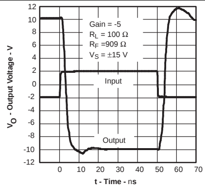
Figure 32. Inverting Large-Signal Transient Response
