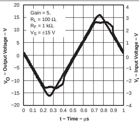
Figure 33. Overdrive Recovery Time
