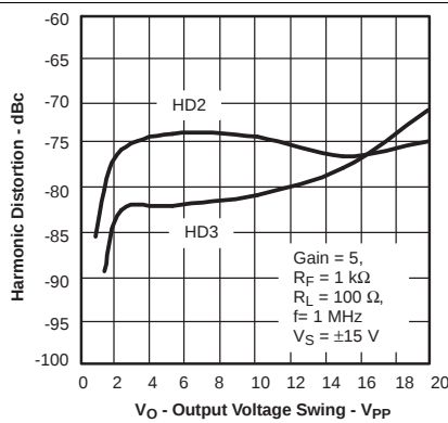
Figure 15. Harmonic Distortion vs Output Voltage Swing
