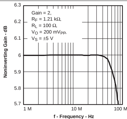
Figure 41. 0.1-dB Gain Flatness Frequency Response
