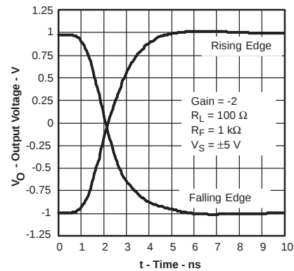
Figure 44. Settling Time
