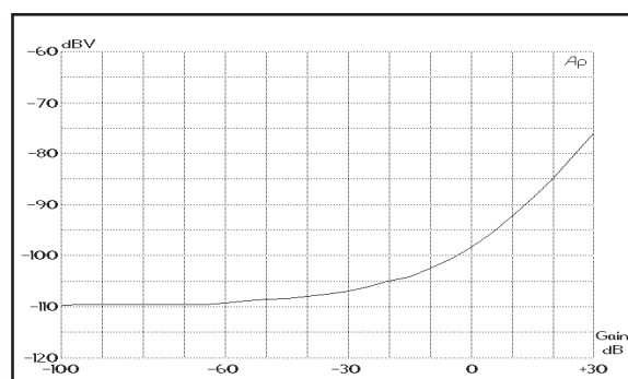
Figure 4. 2181 Series Noise (20kHz NBW) Vs. Gain
