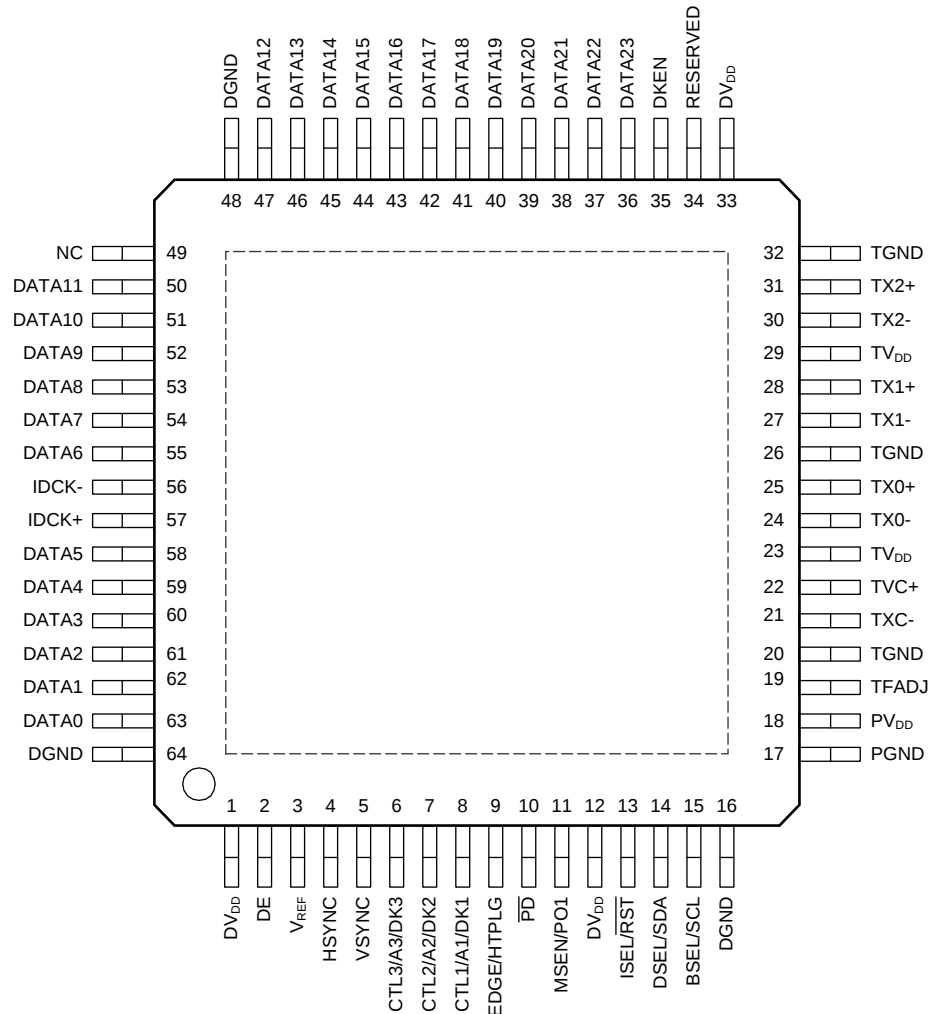
Pin Functions
