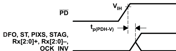
Figure 10. Delay From \overline{PD} Low to High Before Inputs Are Active
