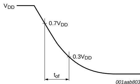
Fig 42. Definition of the fall time of the output signal
