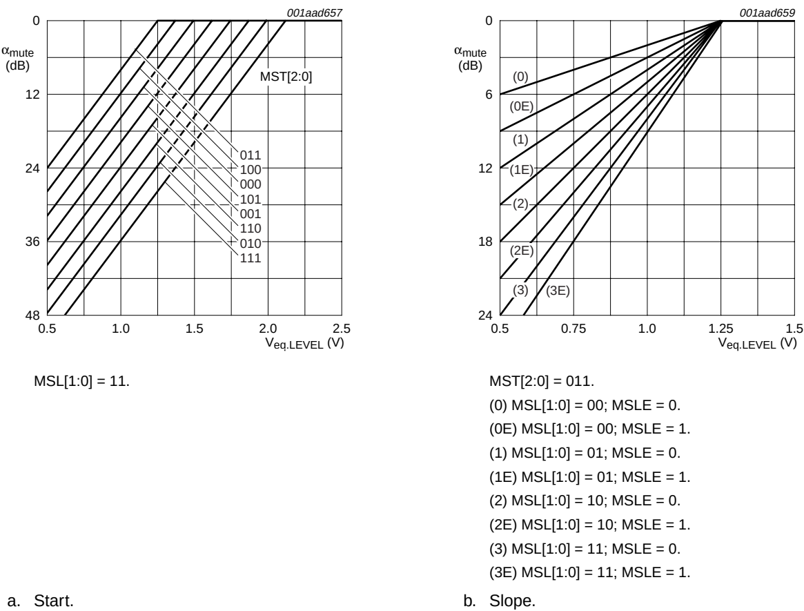
Fig 29. Soft mute start and slope settings versus equivalent level voltage (AM mode)
