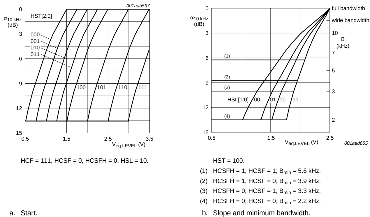
Fig 26. High cut control start and slope settings versus equivalent level voltage; HCC detector (HCMP = 0 for level or HCMP = 1 for level, WAM and USN)
