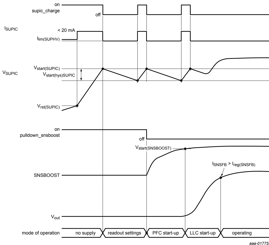
Figure 4. Start-up sequence and normal operation
