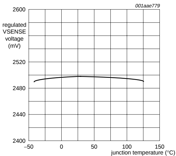
Fig 4. Typical regulated V_{\text{SENSE}} voltage versus junction temperature
