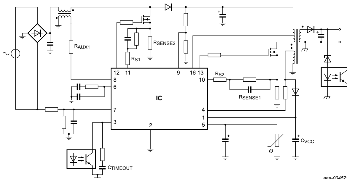
Fig 16. Typical application diagram for the TEA1751T
