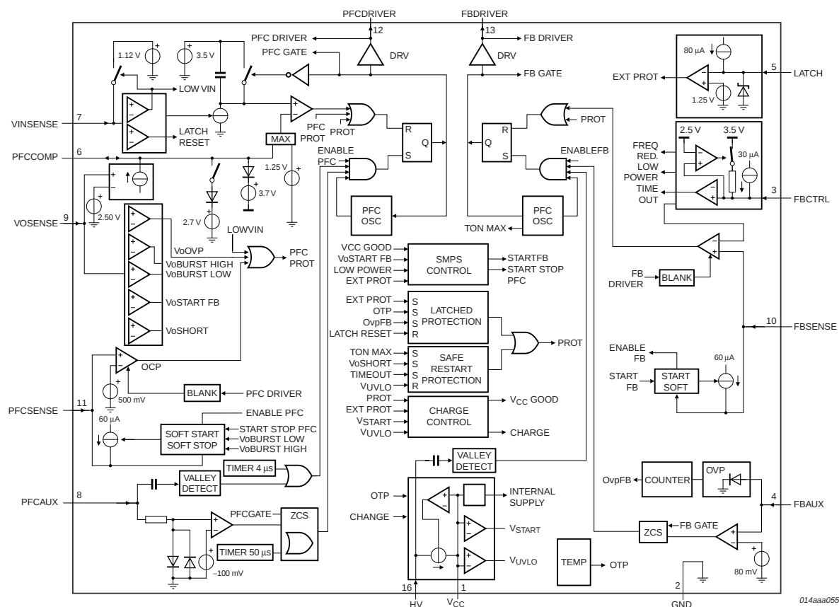
Fig 1. Block diagram
