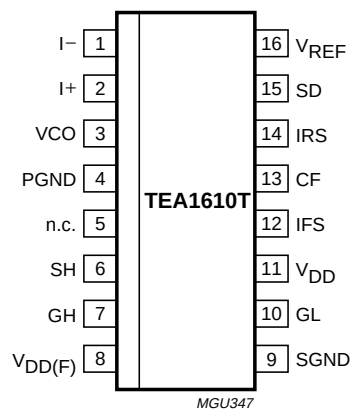
Fig.4 Pin configuration: TEA1610T.
