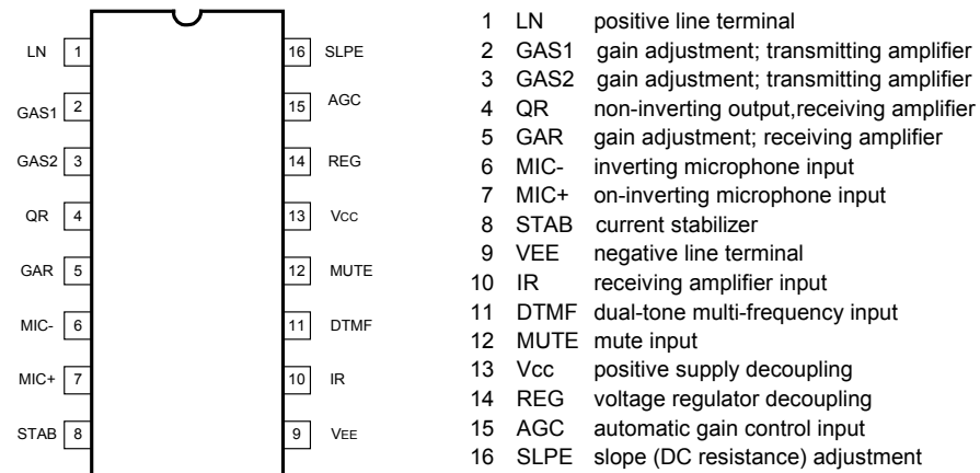
Fig.2 PIN CONFIGURATIONS
