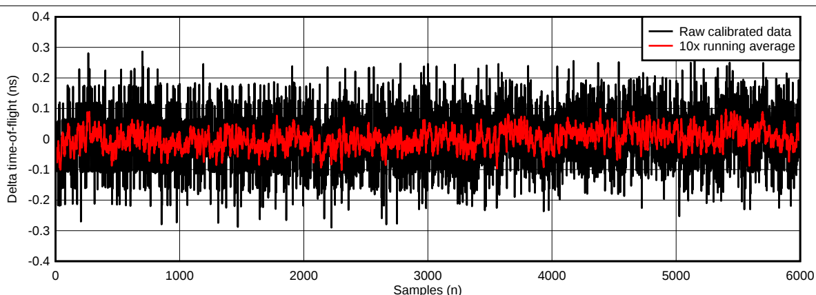
Figure 46. Calibrated Raw and Averaged Delta Time-of-Flight Data
