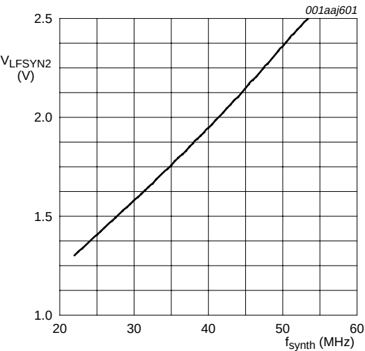
Fig 45. Typical synthesizer loop filter voltage as function of synthesizer frequency
