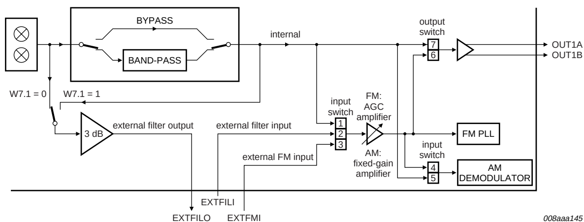
Fig 9. Signal path for intercarrier (2nd SIF) processing
