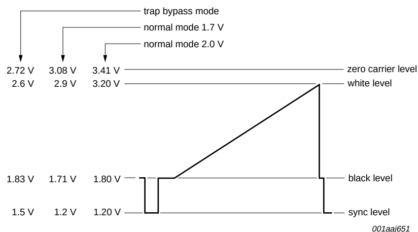
Fig 10. Typical video signal levels on output pin CVBS (sound carrier off)
