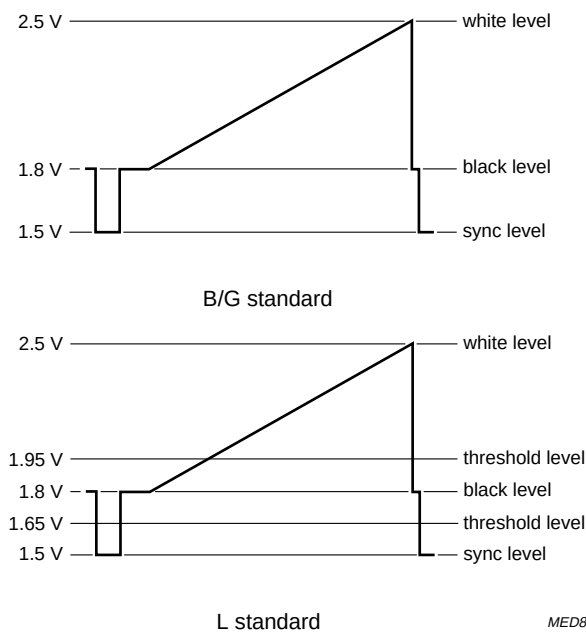
Fig.9 Typical video signal levels on output pin 9 (sound carrier off ).
