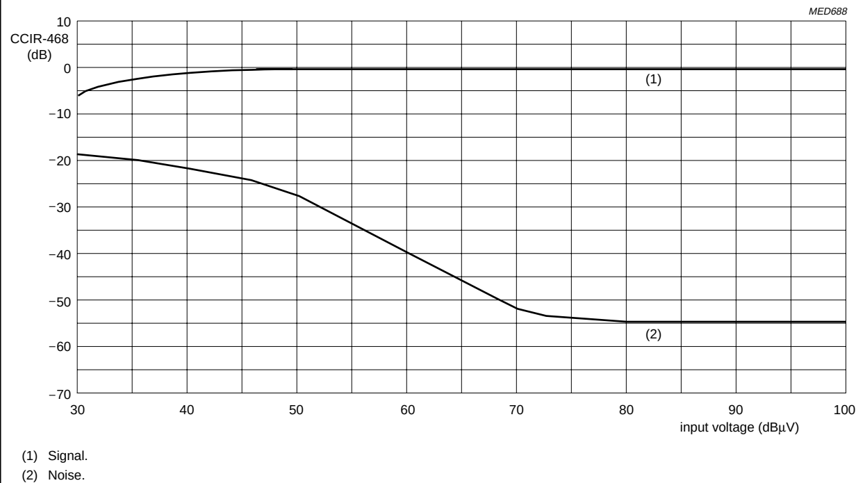
Fig.10 Typical audio signal-to-noise ratio as a function of input signal at AM standard (m = 54%).
