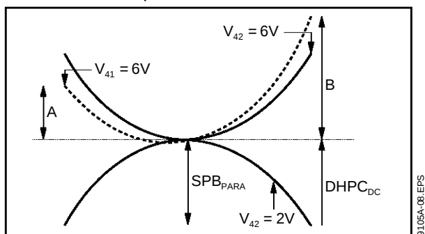
Figure 6 : Dynamic Horizontal Phase Control Output
