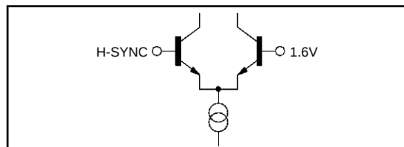
Figure 9 : Input Structure
