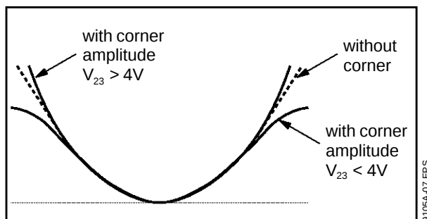
Figure 7 : Vertical Dynamic Focus Function
