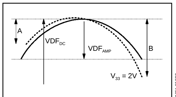
Figure 7 : Vertical Dynamic Focus Function
