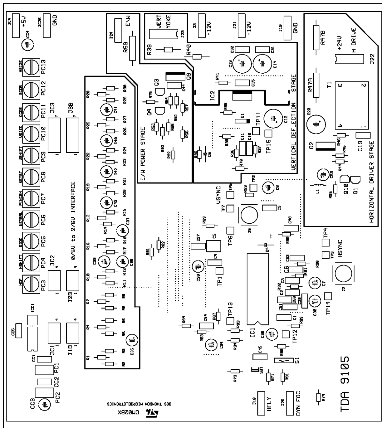
Figure 56 : Components Layout
