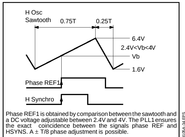
Figure 14 : PLL1 Timing Diagram
