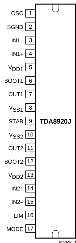
Fig.2 Pin configuration (SOT243-1).
