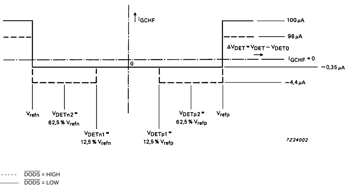
Fig.5 HF gain control current ( I_{GCHF} ) as a function of input voltage \Delta V_{DET} .
