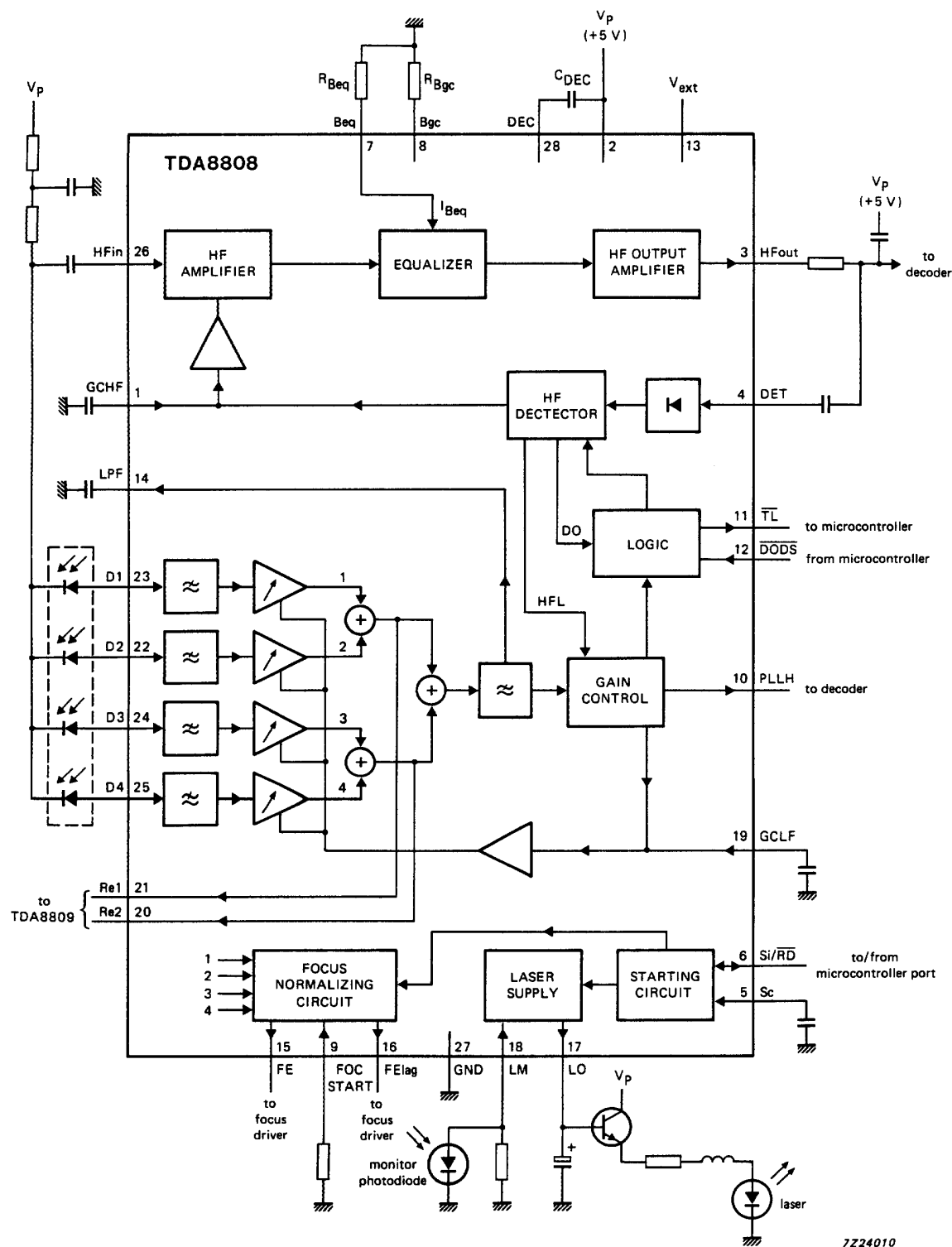
Fig.1 Block diagram.
