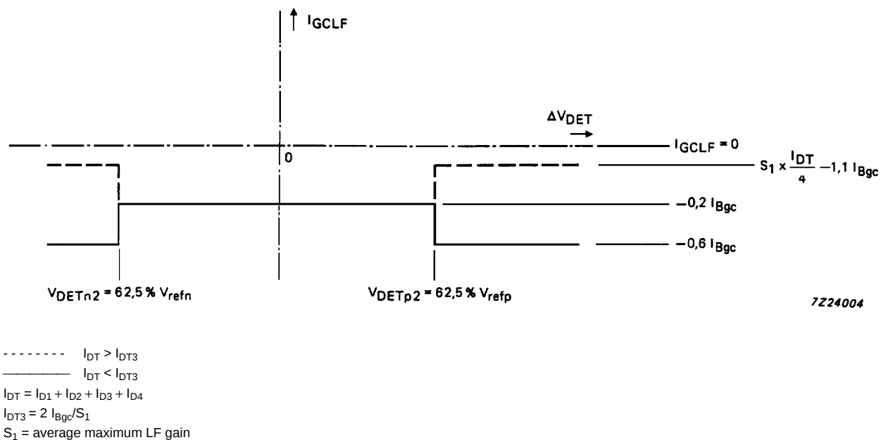
Fig.7 LF gain control current ( I_{GCLF} ) as a function of input voltage \Delta V_{DET} .
