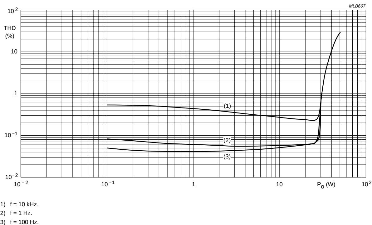
Fig.8 Total harmonic distortion as a function of output power; V P = 14.4 V; R L = 2 Ω.
