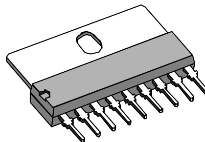
SIP9 (Plastic Package) ORDER CODE: TDA8133
