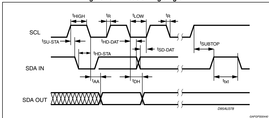
Figure 18. I 2 C bus timing diagram
