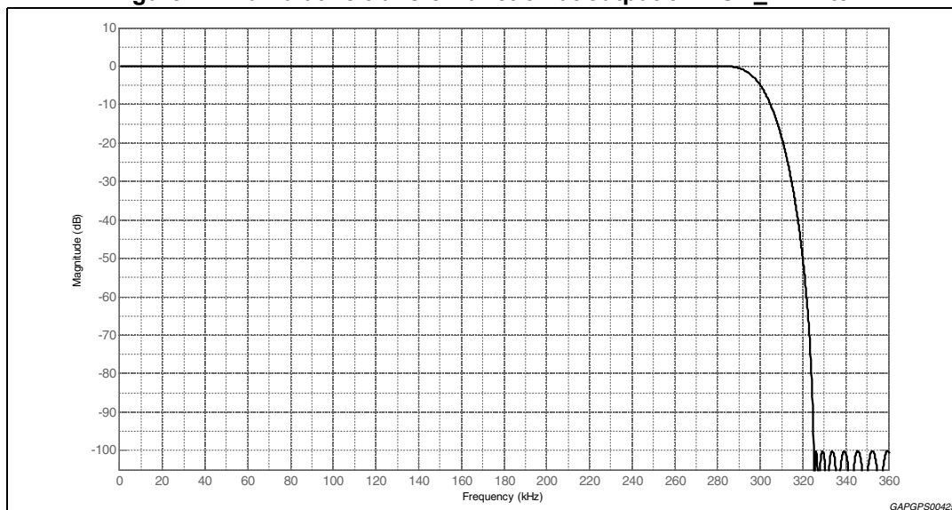
Figure 14. Cumulative transfer function at output of IBOC FM filter
