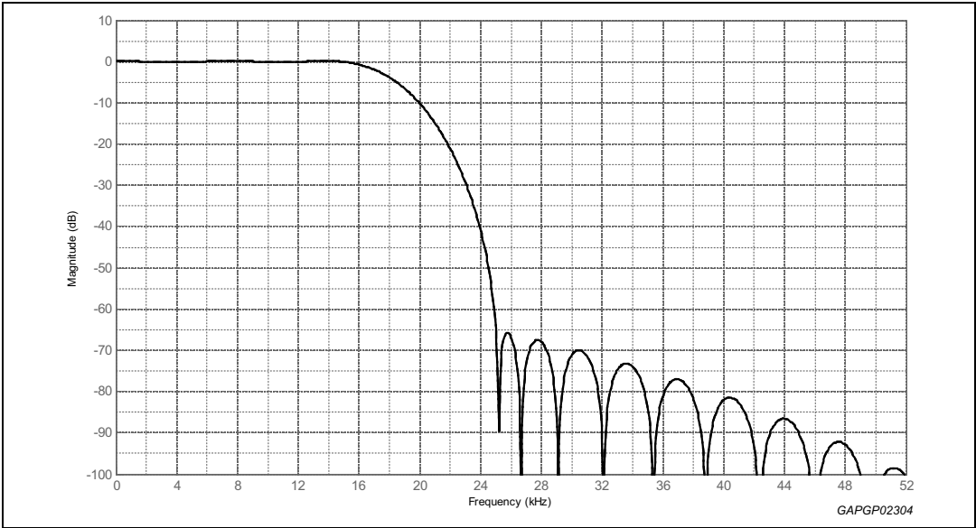
Figure 15. Cumulative transfer function at output of IBOC_AM filter
