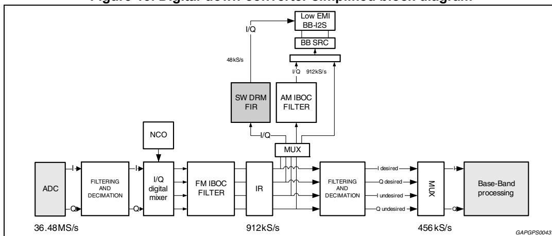
Figure 13. Digital-down-converter simplified block diagram
