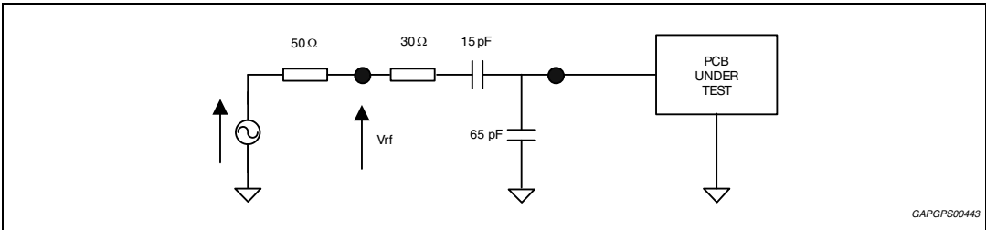
Figure 21. AM LW input set-up
