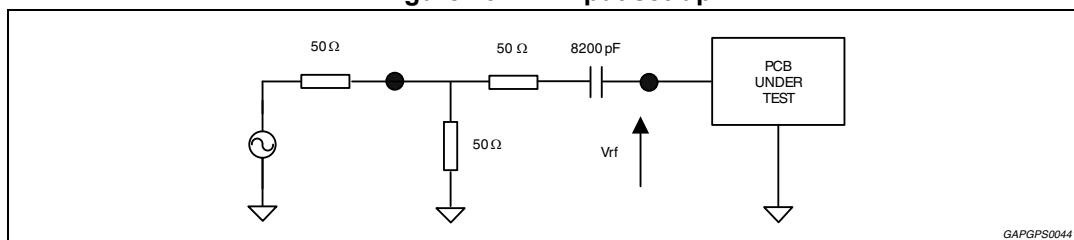
Figure 19. FM input set-up
