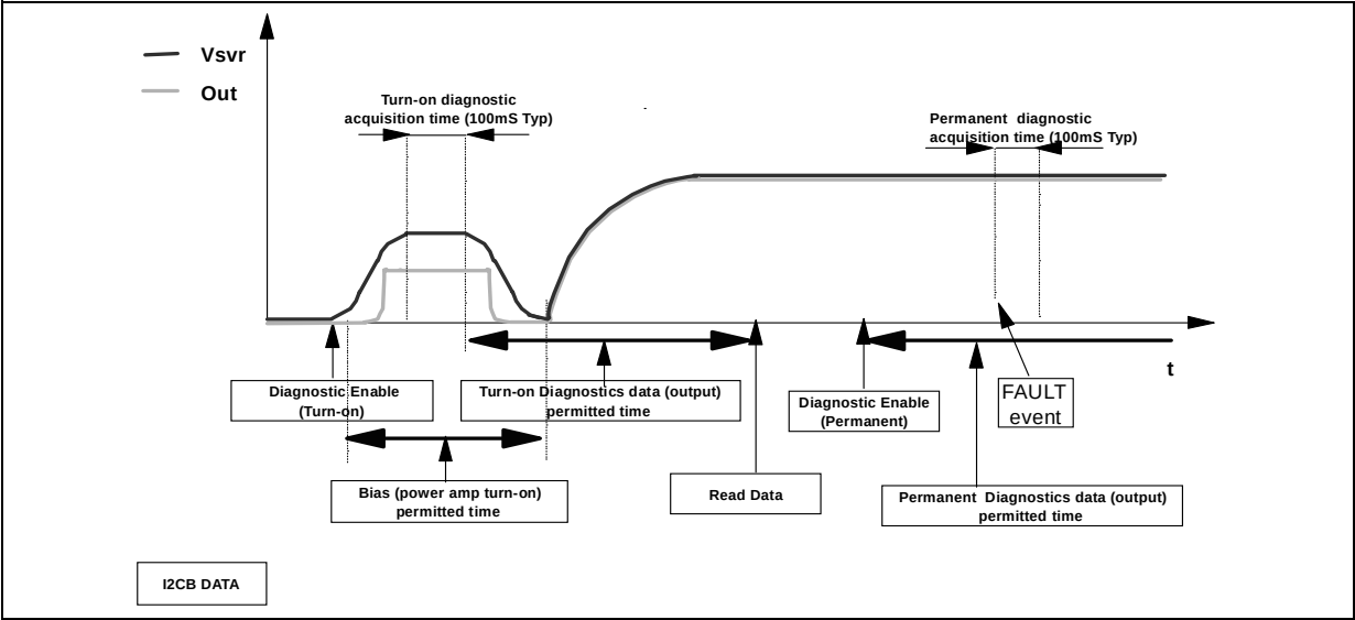
Figure 16. SVR and Output pin behaviour (CASE 2: with turn-on diagnostic)
