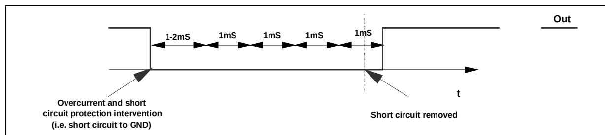
Figure 18. Restart timing with Diagnostic Enable (Permanent)
