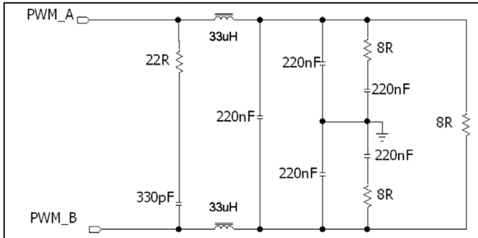
Figure 24: Typical LC filter for an 8 \Omega speaker
