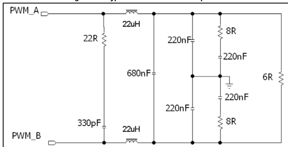
Figure 25: Typical LC filter for a 6 \Omega speaker
