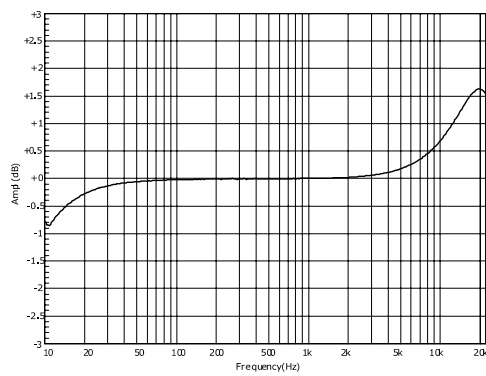
Figure 16: Frequency response
