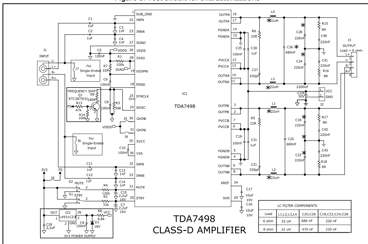
Figure 3: Test circuit for characterizations
