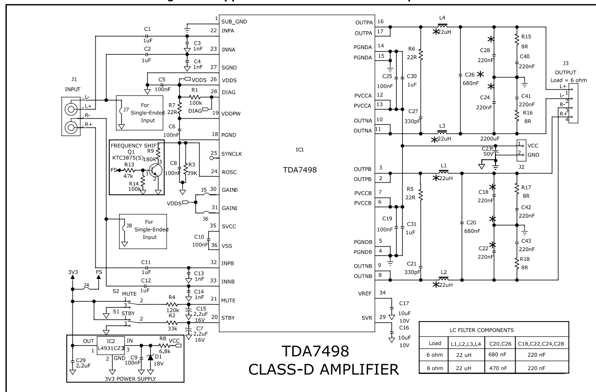
Figure 19: Application circuit for 6 \Omega or 8 \Omega speakers
