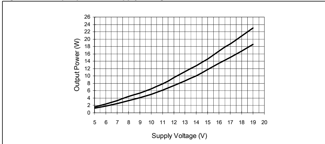
Figure 3. Output power vs supply voltage
