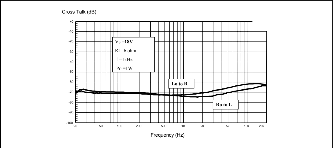
Figure 17. Cross talk vs frequency
