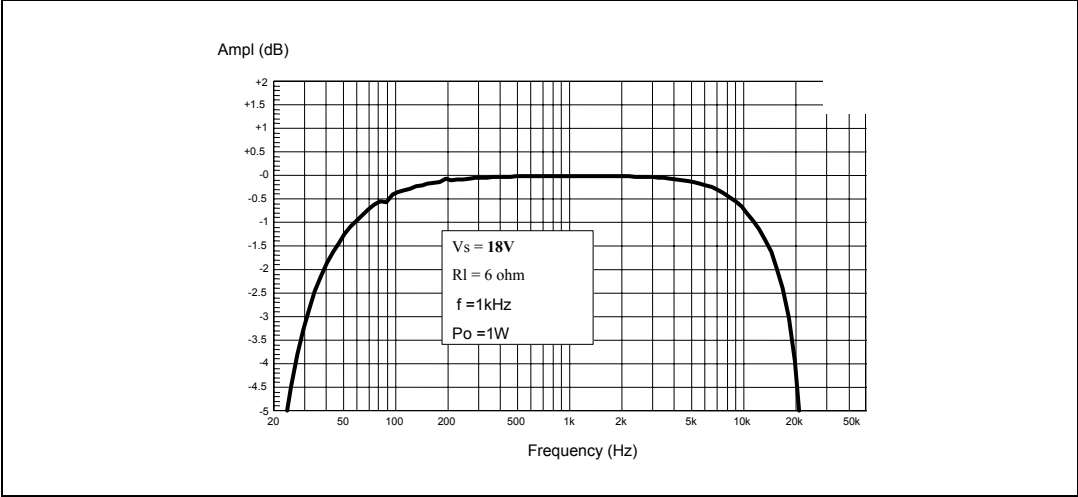
Figure 15. Frequency response
