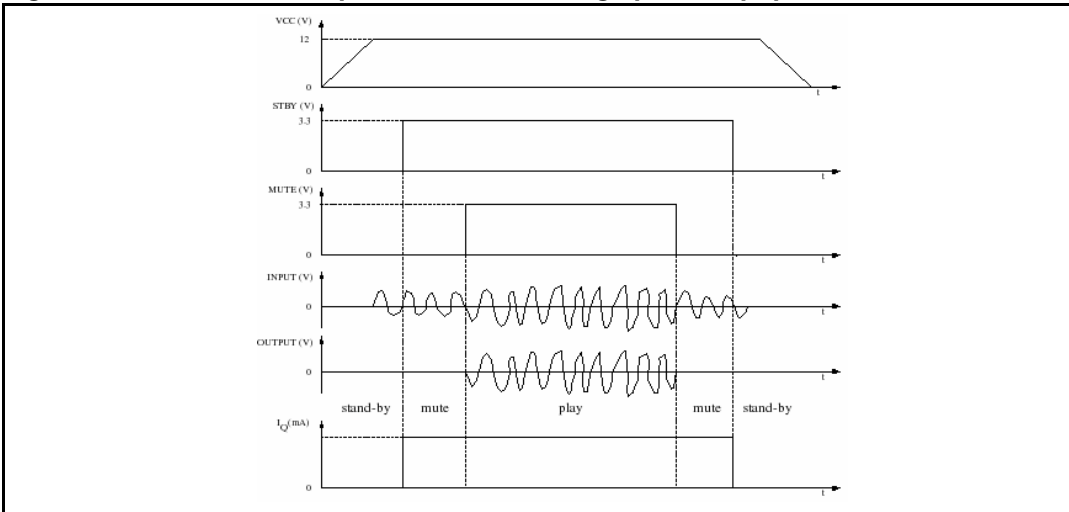
Figure 24. Turn on/off sequence for minimizing speaker “pop”
