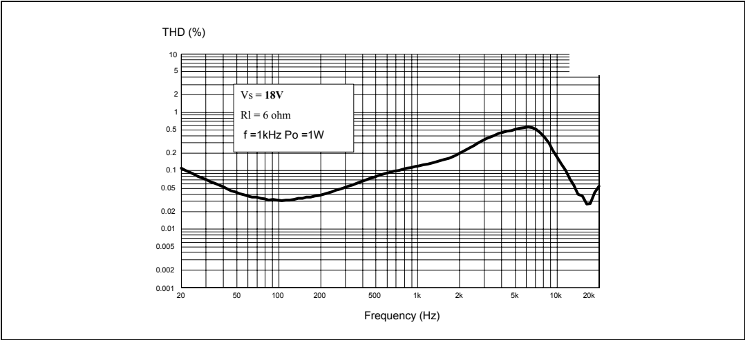
Figure 16. THD vs frequency
