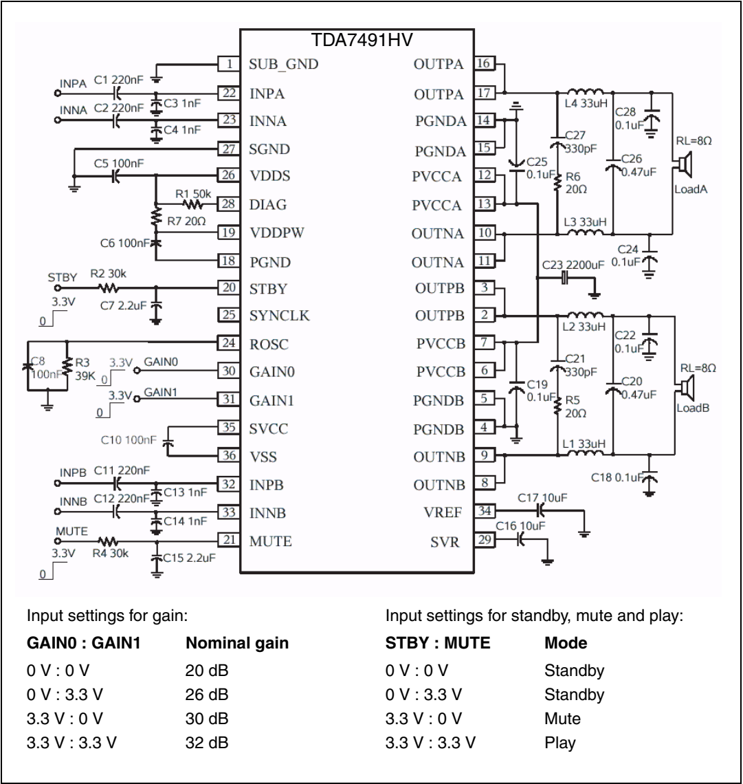
Figure 22. Application circuit
