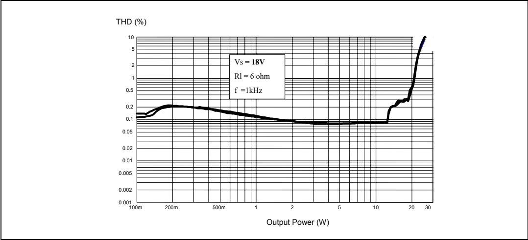
Figure 14. THD vs output power
