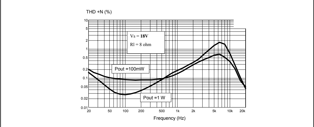
Figure 6. THD + N vs frequency
