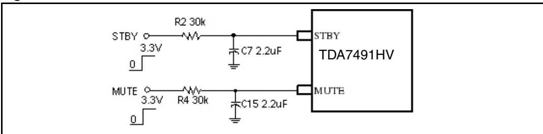
Figure 23. STBY and MUTE circuit
