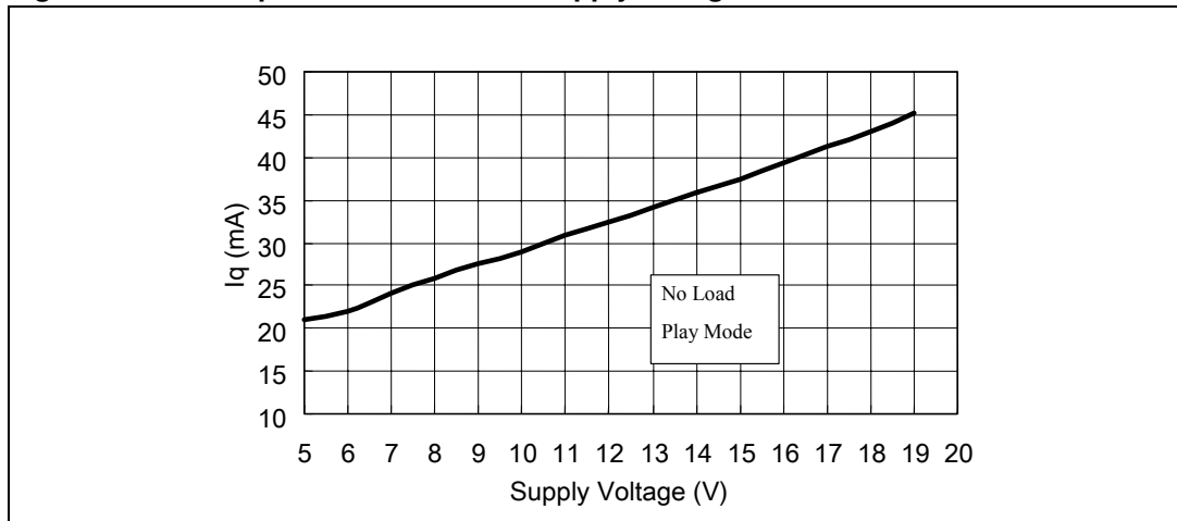
Figure 11. Total quiescent current vs supply voltage
