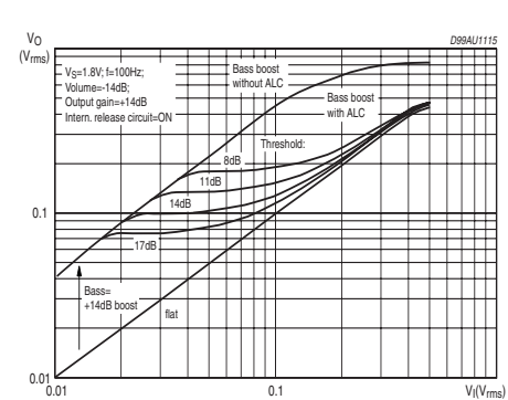
Figure 12. BASS ALC: Threshold curve
