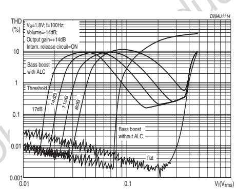
Figure 13. BASS ALC: THD
