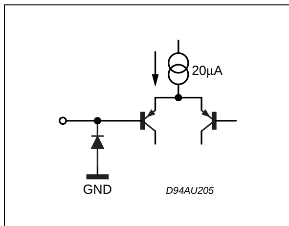
Figure 17. Pin: SCL, SDA
