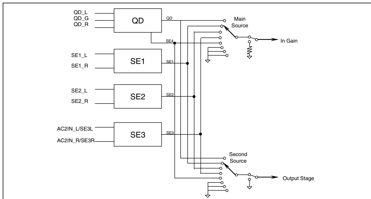
Figure 4. Input Stage
