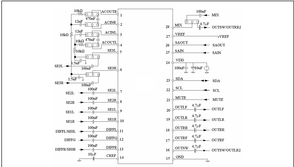
Figure 25. Test Circuit
