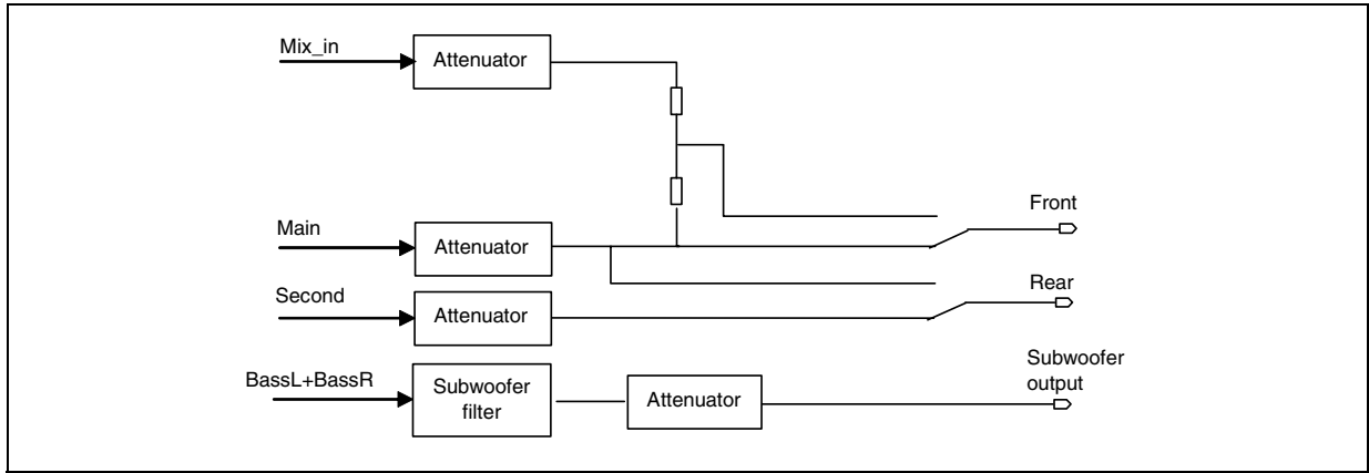
Figure 24. Output Selector
