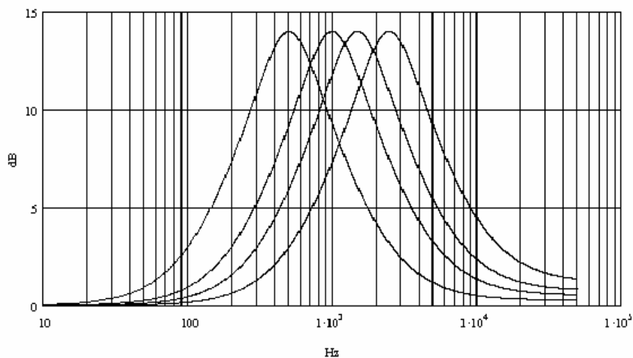
Figure 15. Middle center Frequencies @ Gain = 14dB, Q = 1
