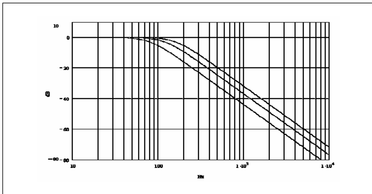
Figure 19. Subwoofer Control
