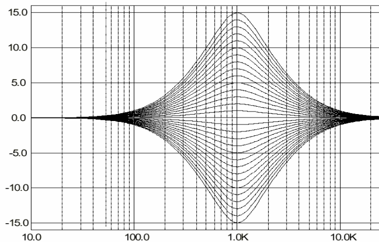
Figure 14. Middle Control @ f_C = 1\text{ kHz} , Q = 1
