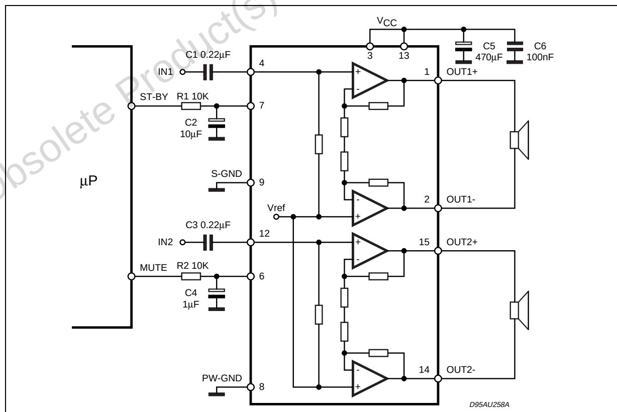
Figure 1. Microprocessor Application
